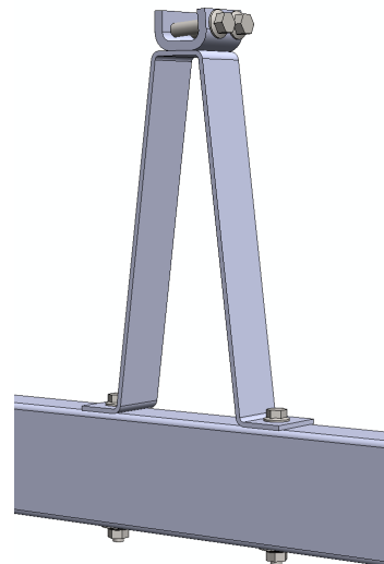
Spine support bracket fixed to bearer
