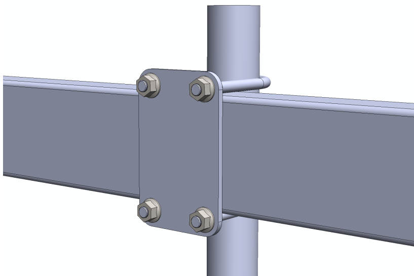
Bearer fixed to post using U-bolts
