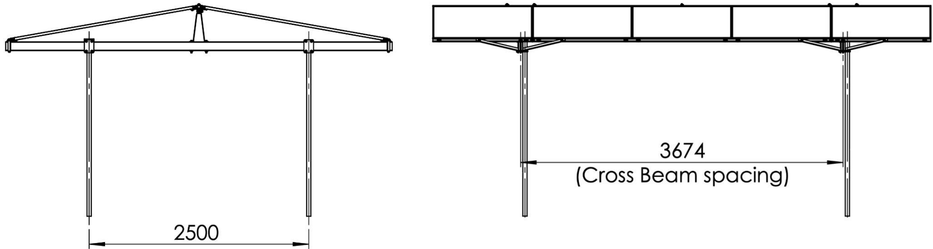
Solpod Ground post spacing
