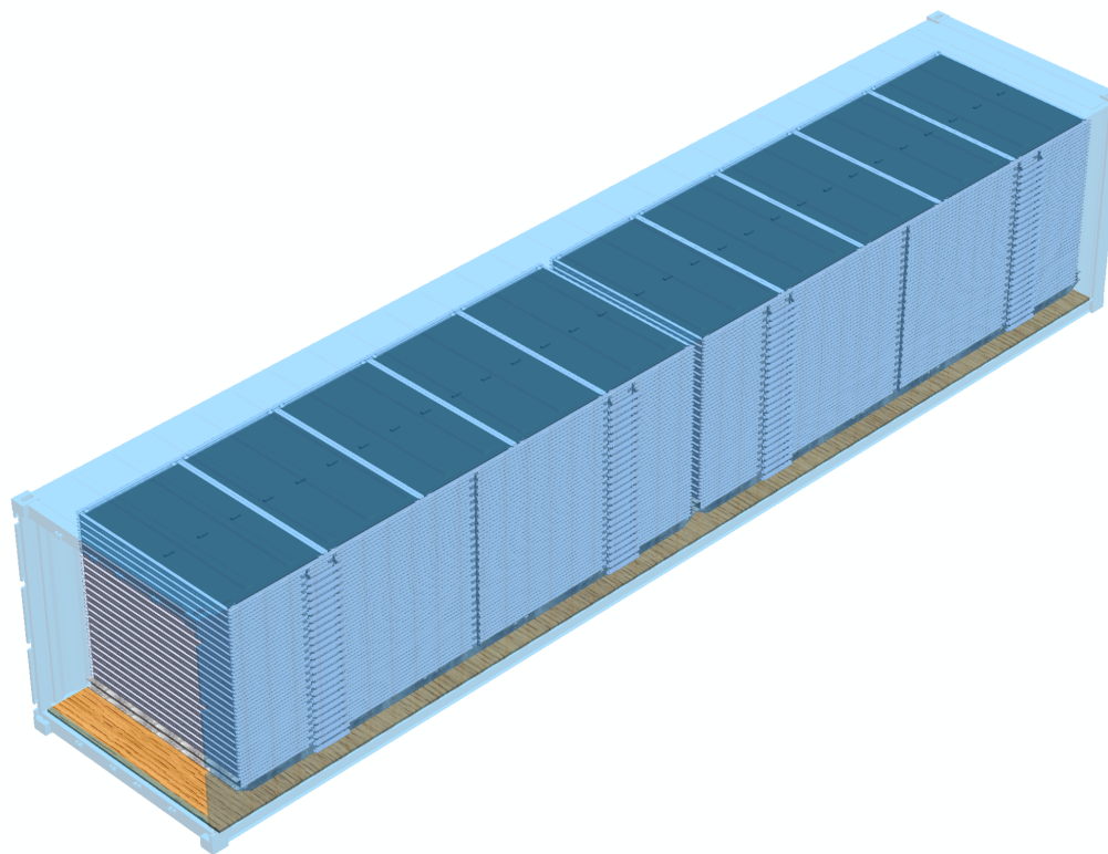
Two stacks of Solpods, on roller skids, in a 40' GP container
