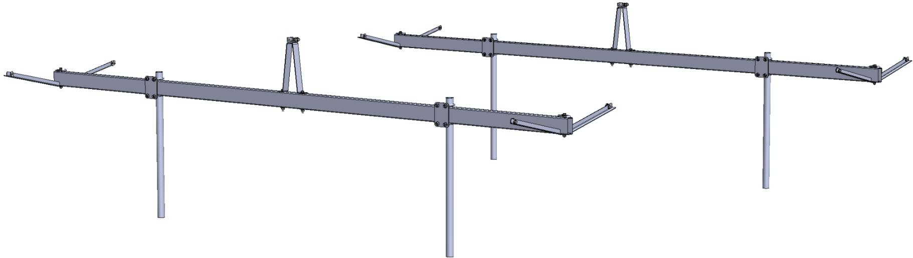
Ground frame showing four rammed posts, two bearers, and two spine support brackets
